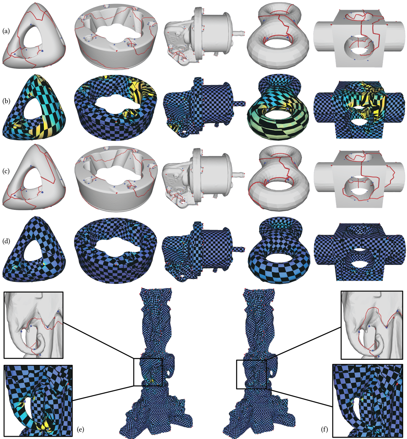
Fig. 10. Comparison of seamless parametrizations on surfaces of non-trivial topology, computed by the bare SP method [Campen et al. 2019] (row b, e) and by our method (row d, f). The used cut graphs are shown in red, the initial hole-chain used for SP (row a, e) and the rerouted version used by our method (row c, f). Notice their topologically differing structure (i.e. they wind around some handles or cones differently), as well as the higher distortion of the results by the bare SP method due to being unable to properly align to the underlying smooth cross-field for topological reasons. Notice that this distortion cannot be reduced further by continuous optimization; there are topological obstacles.
