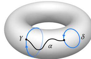
Fig. 6. Illustration for Prop. 1 concerning quasi-additivity of holonomy numbers on loops.
